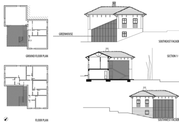
Figure 6. Mountain house – example of reconstructing a house with sunroom
