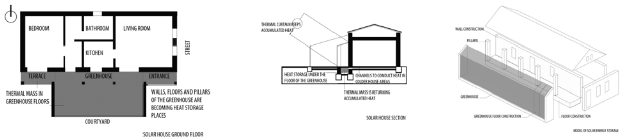
Figure 5. Vojvodina – example of reconstructing a house with sunroom
