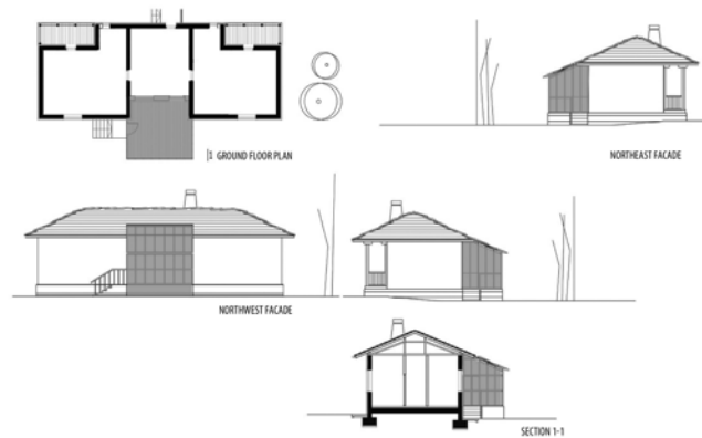
Figure 7. Šumadija and Pomoravlje – example of reconstructing a house with sunroom
