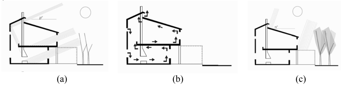
Figure 4. The way a sunroom functions: (a) winter-daytime (b) winter-nighttime (c) summer-daytime [1]
